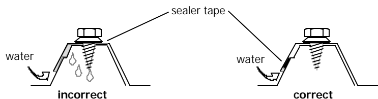
Stitch Screw & Sealer Tape Placement
